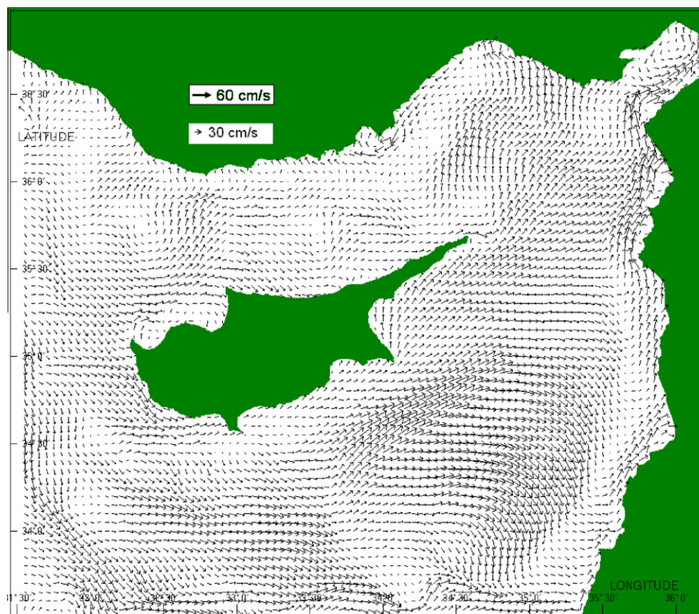
Fig. 6. Surface-currents field for 23 July 2006 at 12:00 from the CYCOFOS forecasting system. Dark arrows represent current directions and intensity in cm/s.
