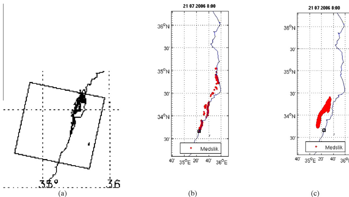
Fig. 8. Panel (a) shows the ASAR ENVISAT image for day 21. The ASAR image is compared with the position of the oil slick as predicted by CYCOFOS (panel b) and by MFS (panel c). (a) July 21 (07:49): ASAR Envisat image. Oil spill (black) is mostly located in the gulf of Beirut but has already reached Chekka, located south of Tripoli. (b) The position of the oil slicks (red) as predicted for 21 July at 8:00 GMT (after 192 h) by CYCOFOS. (c) The position of the oil slicks (red) predicted for 21 July at 8:00 GMT (after 192 h) by MFS. (For interpretation of the references to color in this figure legend, the reader is referred to the web version of this article.)
